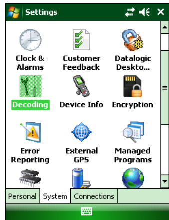
Windows Mobile
